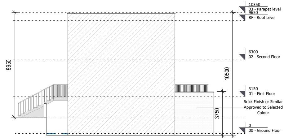
② Left Elevation / Party Wall Section 1 : 200
