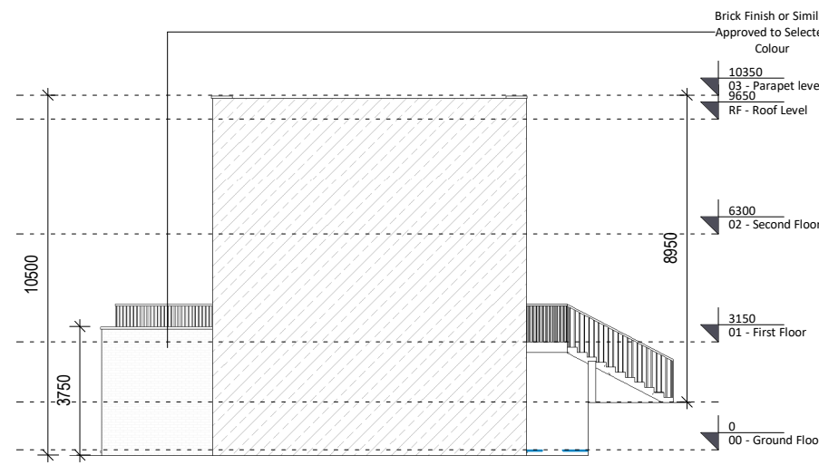
④ Right Elevation / Party Wall Section 1 : 200
